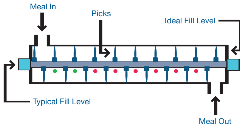
Figure 8: A Single Shaft Conditioner Showing Ideal and Typical Meal Fill Level (courtesy of S Parker)
