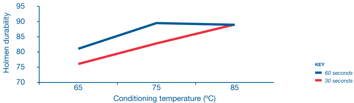
Figure 6: The Effect of Conditioning Temperature and Time on Pellet Durability (Svihus, 2005)
